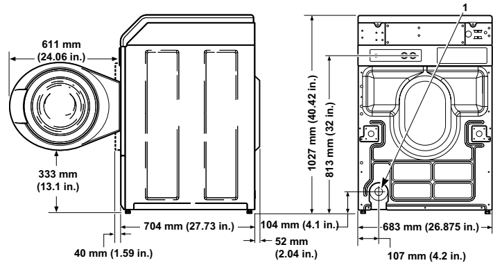
Models With Gravity Drain 1. 38 mm (1.5 in.) Inside Diameter; 47 mm (1.86 in.) Outside Diameter
